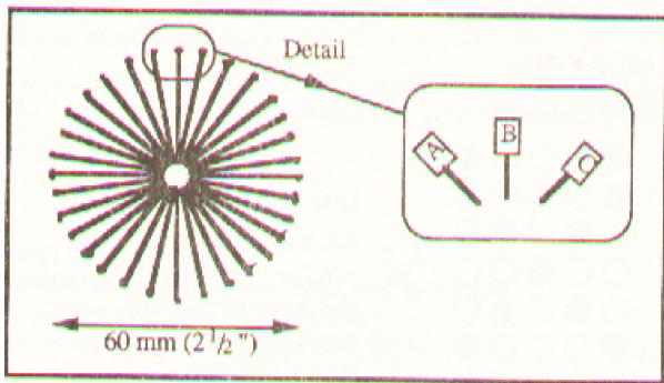
a) The Whole Daisy Wheel b) Detail of the Daisy wheel Spokes
