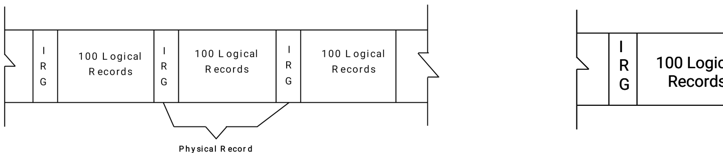
Fig. 2.9.1: Magnetic tape with a Blocking Factor of 100
