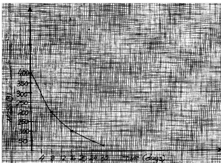
Decay curve of Iodine 131
